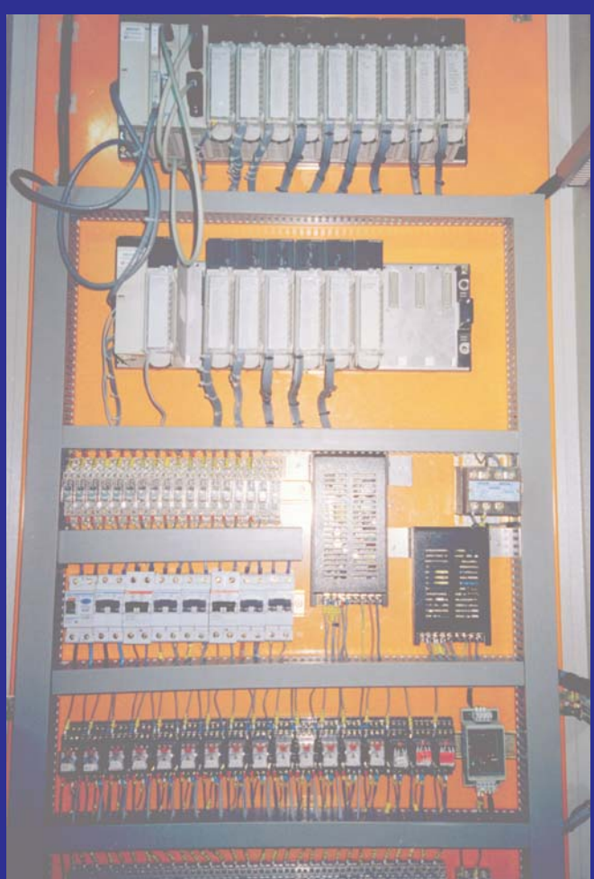
Detail of electrical panel and PLC
